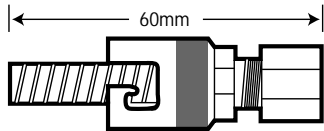
Single slot Cap internal diameter 11.4mm suitable for 3.0mm and 4.5mm diameter probes
