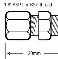
Adjustable Mounting Compression Fittings
