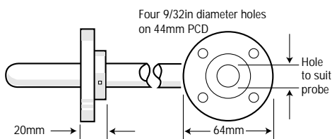
Mounting Flanges for 6.0mm diameter probes
