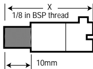
For 3.0mm and 4.5mm bayonet assemblies
