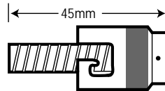
Single slot Cap internal diameter 11.4mm suitable for 3.0mm and 4.5mm diameter probes
