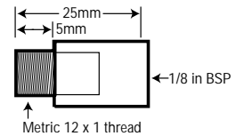
Metric 12 x 1 thread
